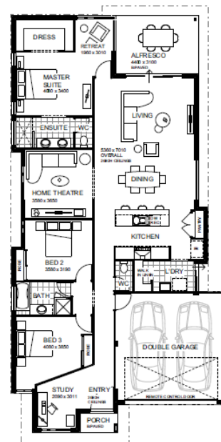
FLOOR PLAN 1:100
