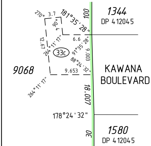
ENLARGEMENT 'A2' Not to scale
