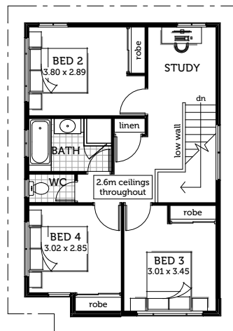
Second storey
